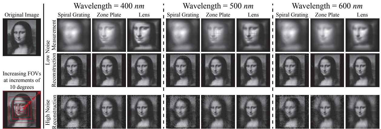
Fig. 3. Reconstructed images by solving the problem in (2), for different incoming light wavelengths and various noise levels for all studied optical elements, presented in Figure 1.
